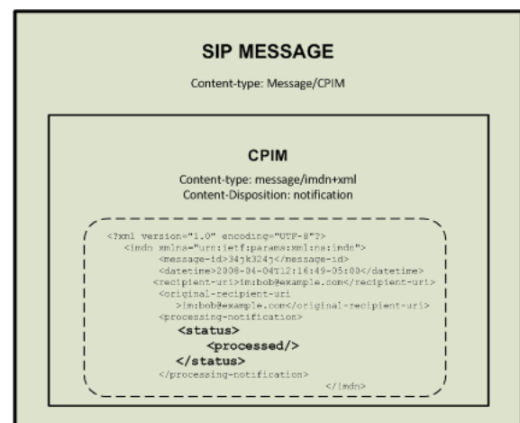
Fig. 7: IMDN for a processed message.
