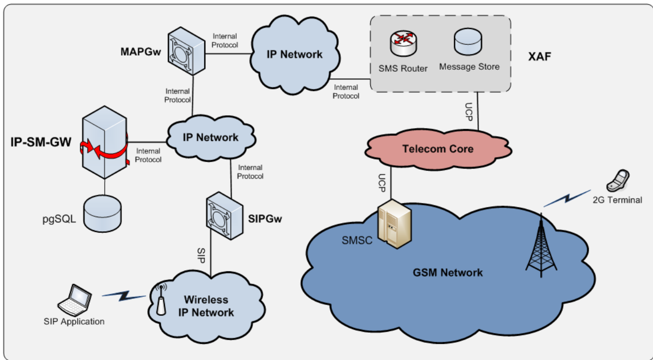
Fig. 8: Created Testbed.
